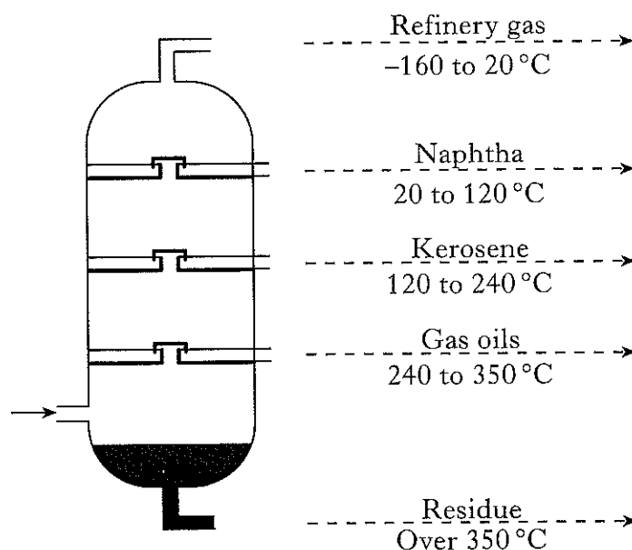
Fraction and boiling point range
